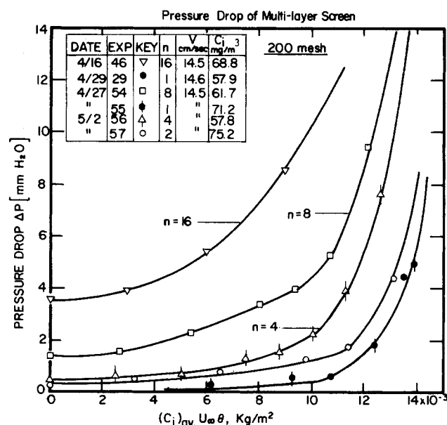
Figure 6. Consistency of experimental data as shown from multilayer model filter results (pressure drop).
