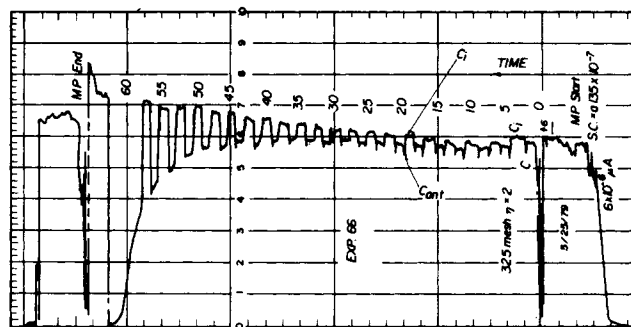
Figure 3. Tyndallometer readings of influent and effluent concentrations.
