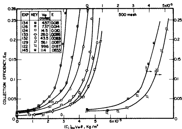
Figure 13. Collection efficiency of single layer model filter at different gas velocities.
