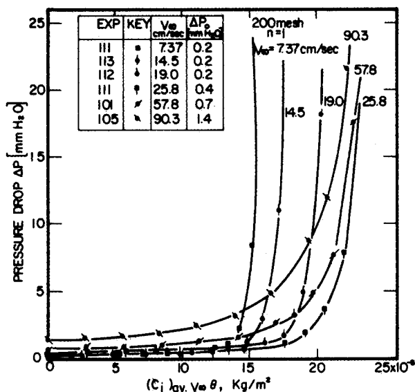
Figure 11. Increase in pressure drop at different air velocities.
