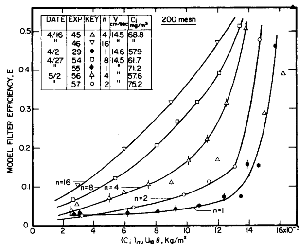
Figure 7. Consistency of experimental data as shown from multilayer model filter results.
