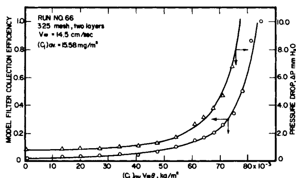
Figure 2. Typical set of model filter measurements.
