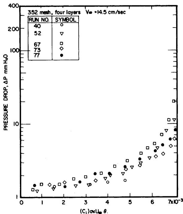
Figure 5. Consistency of pressure drop measurements.
