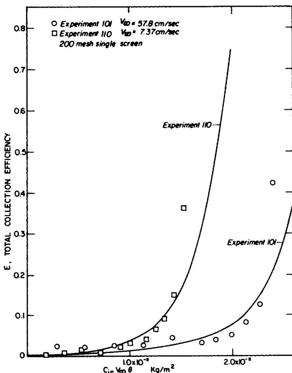
Figure 18. Predictions of single screen model filter performance based on empirical correlations developed in this work and their comparison with data.
