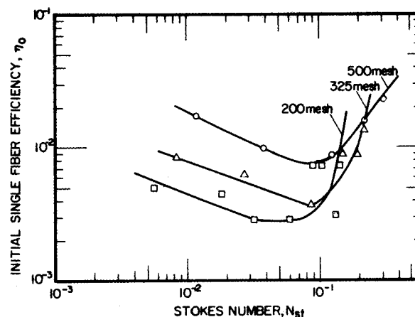
Figure 9. Single fiber collection efficiency of wire screen experimentally determined during initial stage.
