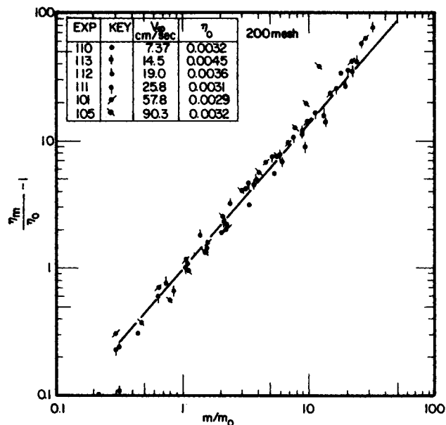
Figure 15. \left(\frac{\eta}{\eta_o} - 1\right) vs. \left(m/m_o\right) .
