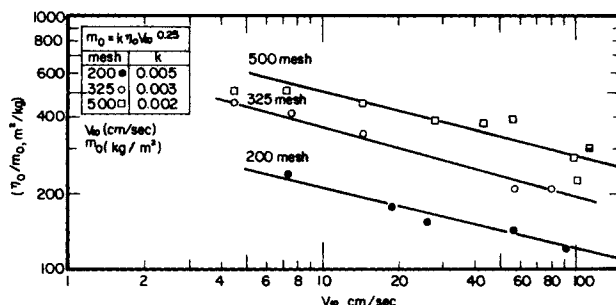
Figure 16. Relationship between m_o and V_\infty .
