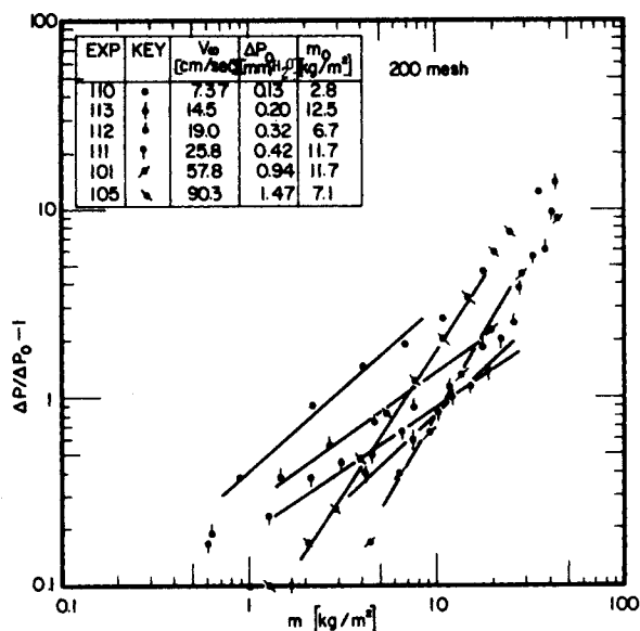
Figure 17. Pressure drop increase vs. m (200 mesh).
