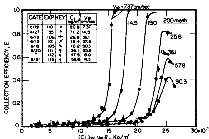
Figure 10. Change of collection efficiency with flow velocity.
