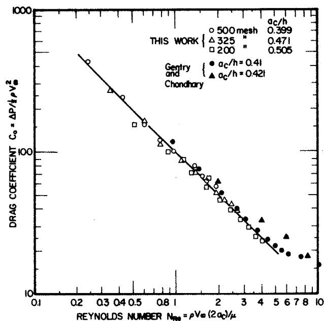
Figure 8. Drag coefficient of wire screen.
