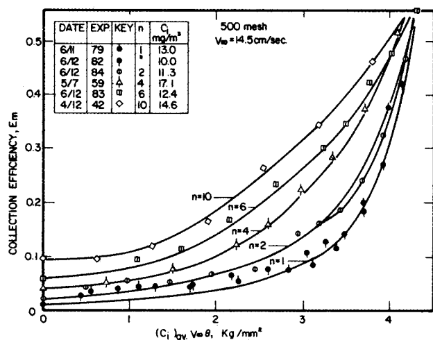
Figure 12. Efficiency of multi-layers model filters.
